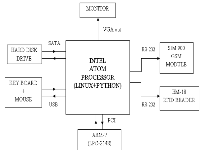
Figure 1: Block Diagram and System Description
