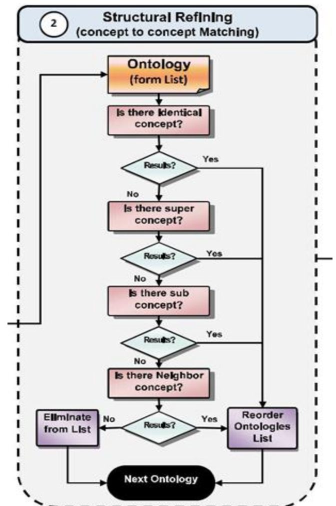
Fig. 4. Structural of the OSSE.
