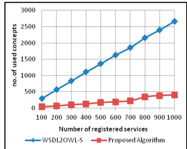
Fig. 6. No. of used concepts versus no. of registered services.
