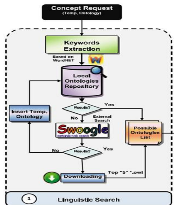
Fig. 3. Linguistic of the OSSE.
