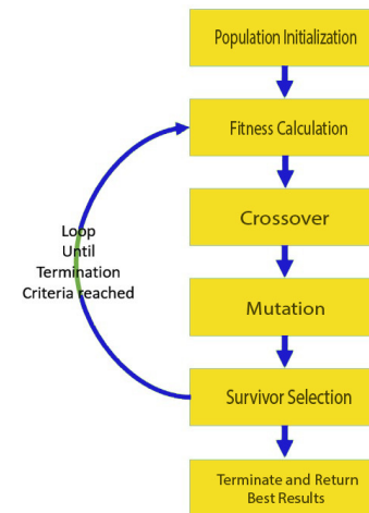
Figure 1. Flowchart of GA System
