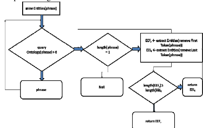
Figure 1: Ontology constriction process
