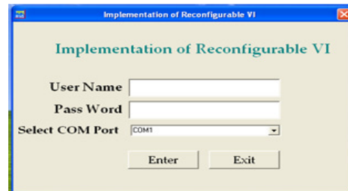
Figure 4: User Window
