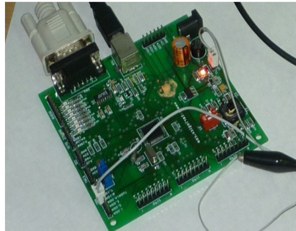
Figure 9:ARM LPC 2148
