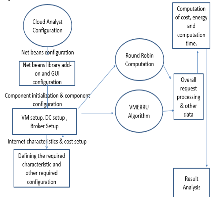
Figure 2: Algorithm Architecture of Complete Workflow.
