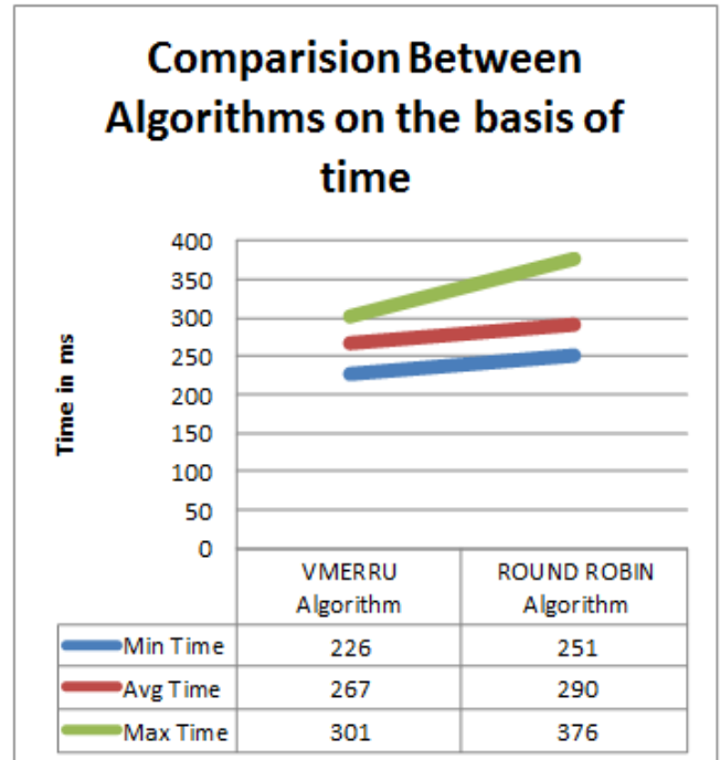
Figure 3: Comparison of algorithm VMERRU Vs Round Robin Scheduling.
