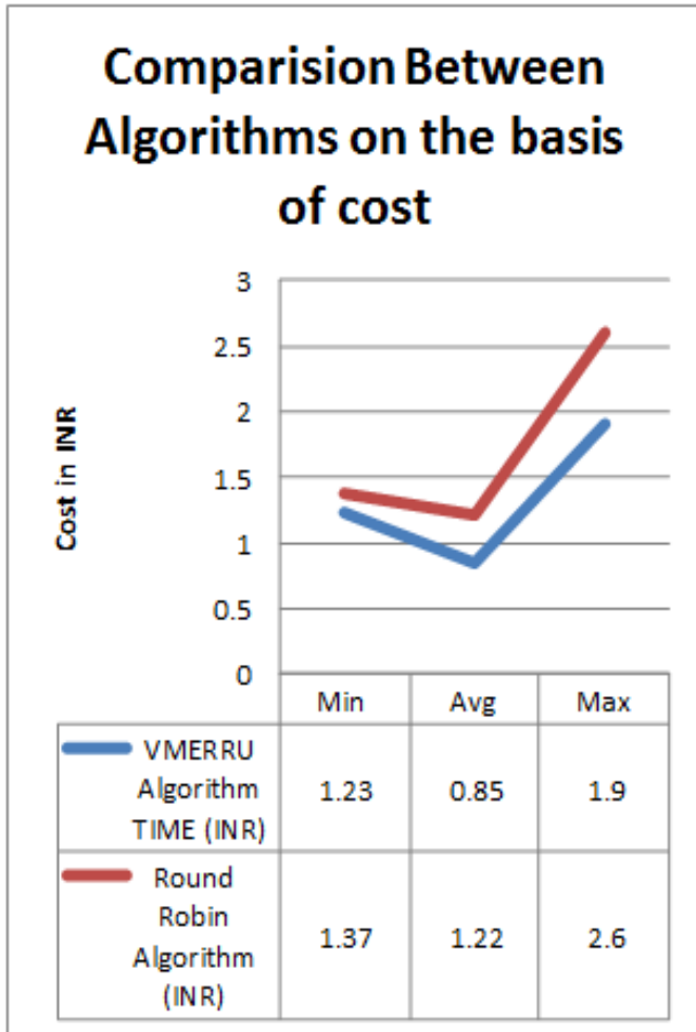
Figure 4: Comparison of algorithm VMERRU Vs Round Robin Scheduling using cost.
