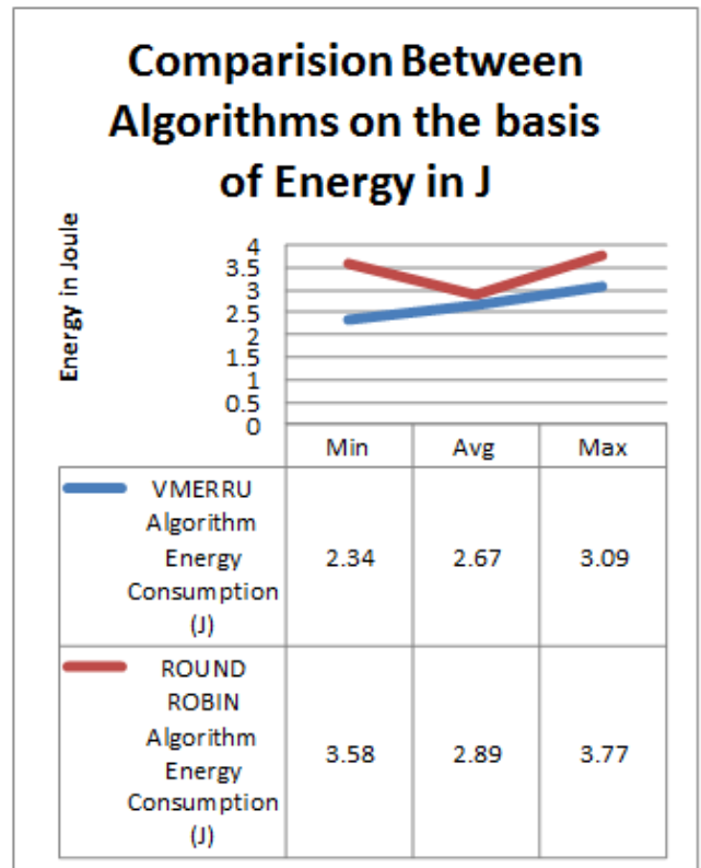
Figure 5: Comparison of algorithm VMERRU Vs Round Robin Scheduling using Energy computation & Utilization.
