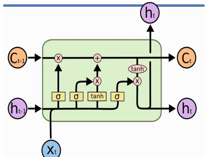
Fig 2: LSTM[8]
