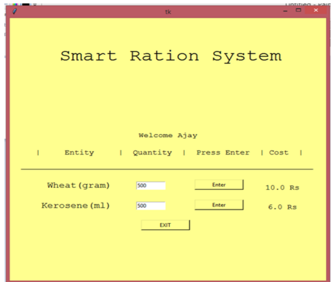
Fig.3. Software Module
