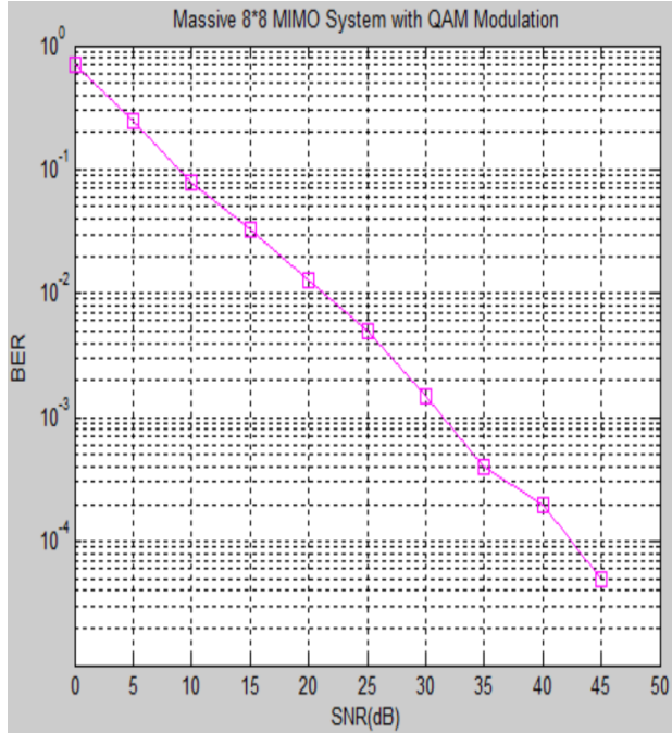
Figure 6: BER vs SNR for Cell free Massive 8x8 System with QR-RLS based Channel Estimation Technique
