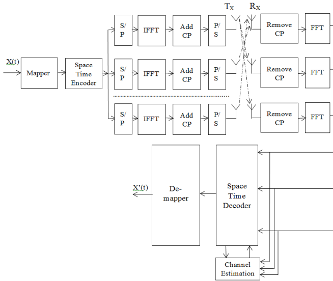
Figure 5: Massive MIMO System Models with Channel Estimation Technique
