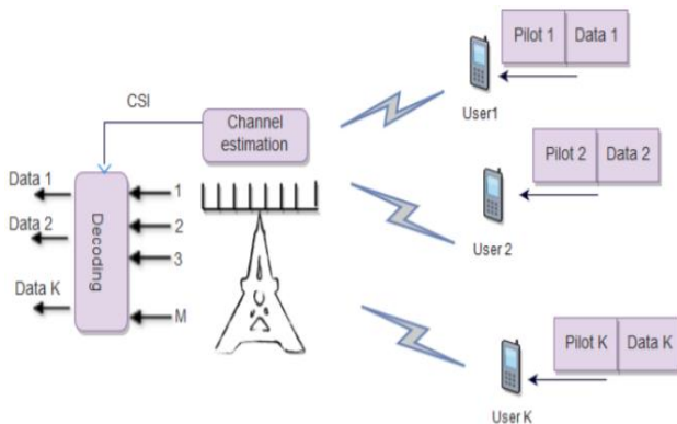
Figure 2: Uplink transmission in a TDD Massive MIMO system
