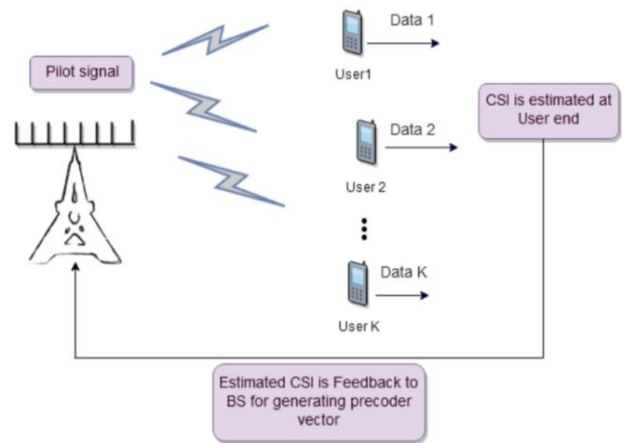
Figure 4: Downlink transmission in an FDD Massive MIMO system
