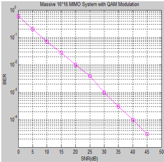
Figure 7: BER vs SNR for Cell free Massive 16x16 System with QR-RLS based Channel Estimation Technique
