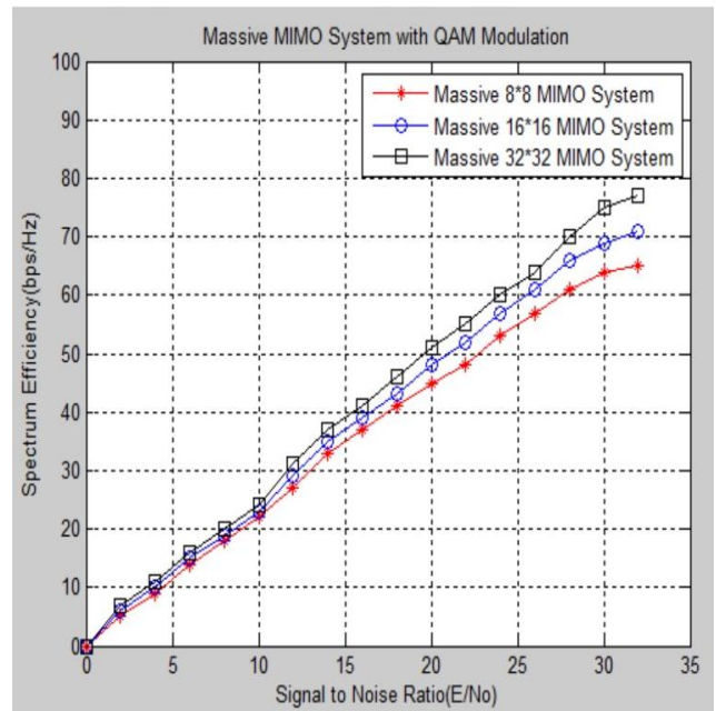
Figure 9: Spectrum Efficiency vs SNR for Cell free Massive 8x8 System with QR-RLS based Channel Estimation Technique
