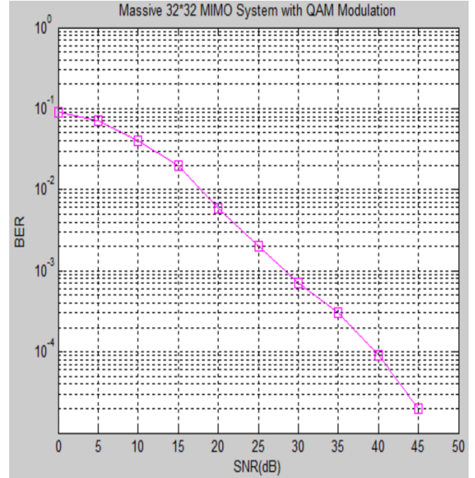
Figure 8: BER vs SNR for Cell free Massive 32x32 System with QR-RLS based Channel Estimation Technique
