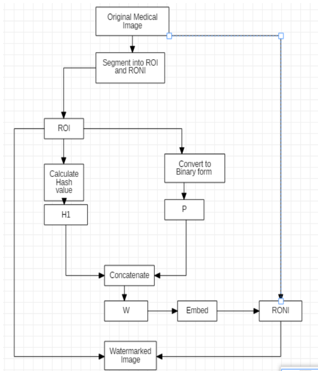
Fig 1: Block diagram of embedding algorithm
