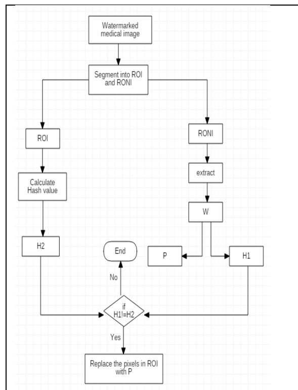
Fig 2: Block diagram of extraction algorithm
