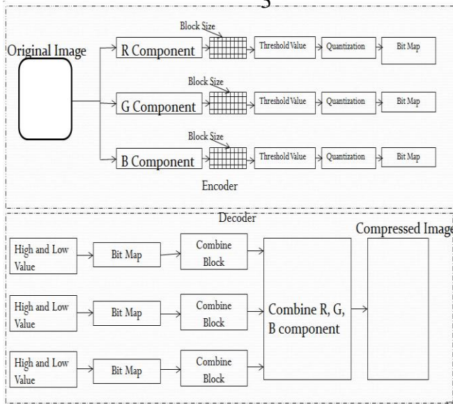
Figure 2: Block Diagram of Proposed Algorithm
