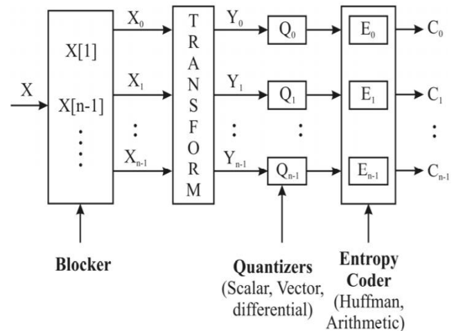
Figure 1: Transform-based image compression system
