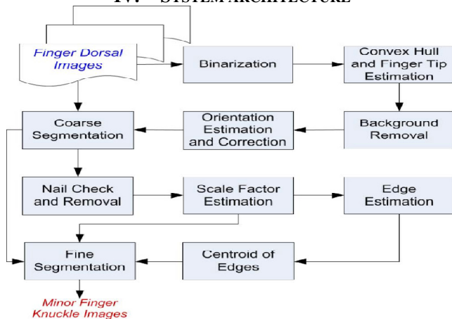
Fig.1. Simplified block diagram of key steps in the automated segmentation of minor finger knuckle images from the finger dorsal images.
