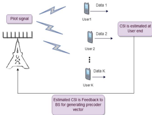
Figure 5: Downlink transmission in an FDD Massive MIMO system
