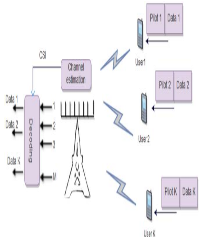
Figure 3: Uplink transmission in a TDD Massive MIMO system
