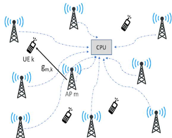
Figure 2: Cell free massive MIMO system
