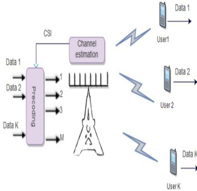
Figure 4: Downlink transmission in a TDD Massive MIMO system
