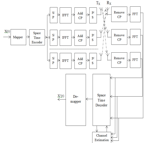
Figure 6: Massive MIMO System Models with Channel Estimation Technique
