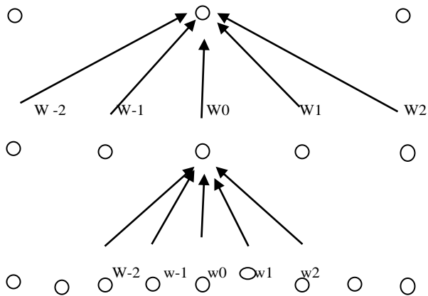
Figure 6. The 5 by 5 pattern generation of Gaussian Pyramid
