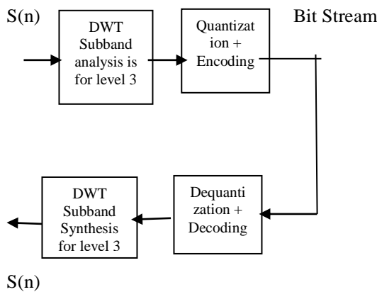
Figure 11. Three Level Image Compression System using DWT
