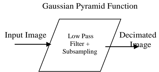
Figure 5. The structure of Gaussian Pyramid
