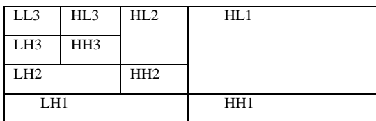
Figure 10. DWT Subband analysis is for level 3
