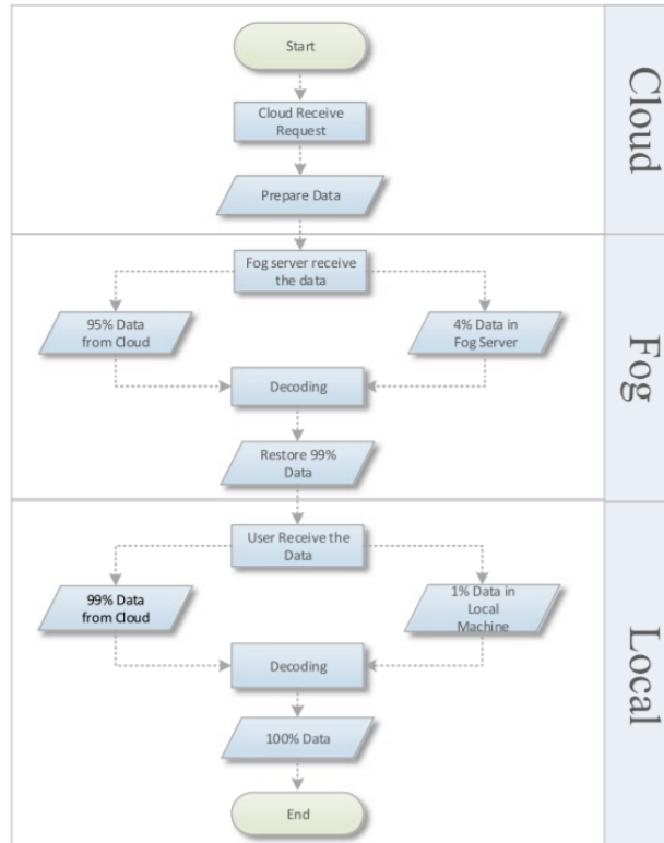
Fig. 7 Diagram of download procedure
