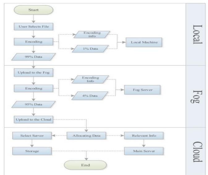
Fig. 6 Diagram of stored procedure
