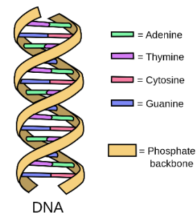
Fig. 3 Double Stranded DNA
