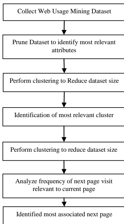
Figure 1: Basic Structure of Web Page Prediction
